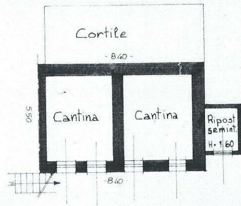
PIANO TERRA H = 2.50
