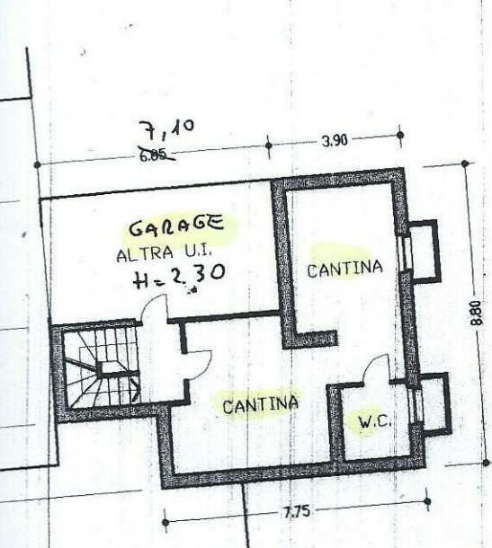
Piano interrato H. Piano 2.30 H = 2.30
