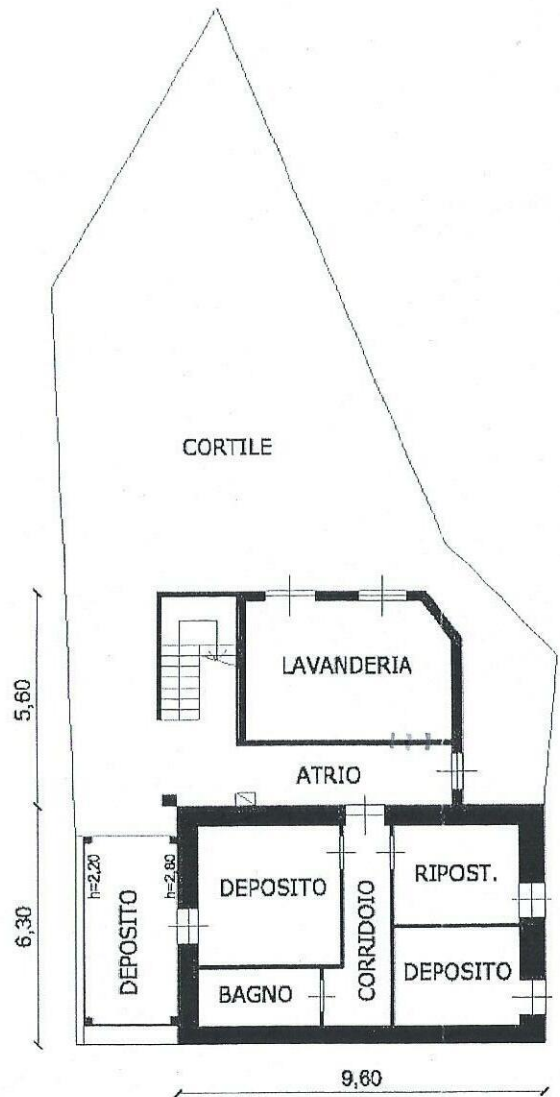
PIANO TERRA H = 2.50
