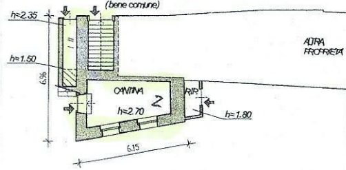
PIANO TERRA - (T)
